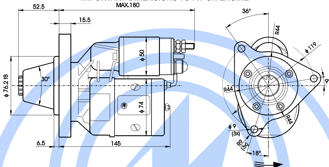
IMPORTANT DIMENSIONS TO FIT ON ENGINE MAX.180
